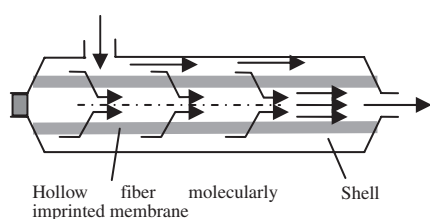
Figure 3. Solution transport in dead-end hollow fiber membrane module.
